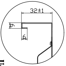
U-shaped Crossmember
